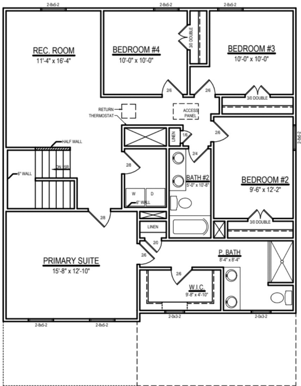
SECOND FLOOR PLAN 1/4" = 1'-0" CEILING HT. = 8'-0"
